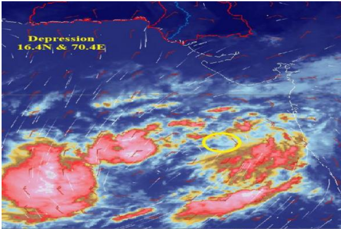
Satellite image (25 October 2025, 1130 PST)
