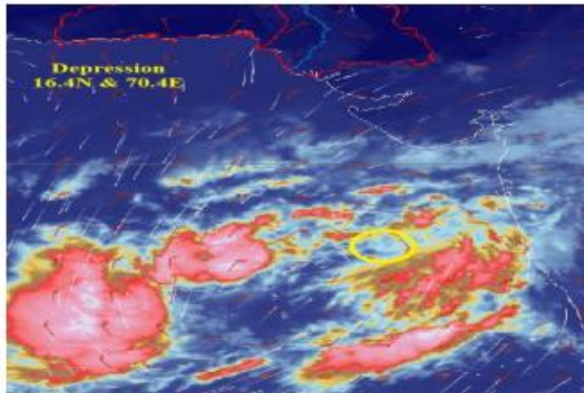
Satellite image (25 October 2025, 1130 PST)
