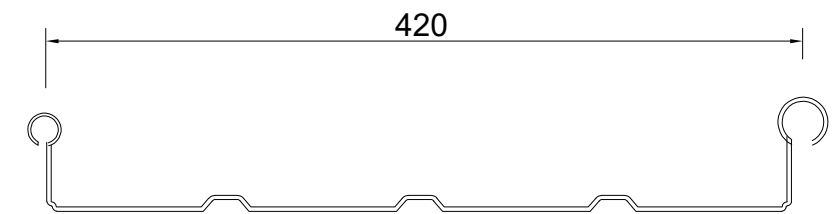
RECO STANDING SEAM LOCK SHEETING
