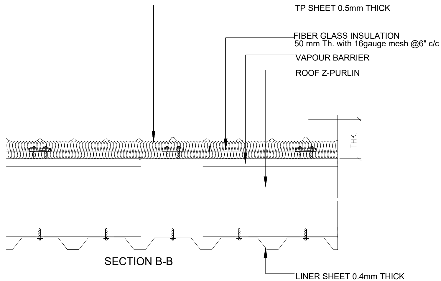
TYP. ROOF SHEETING DETAIL
