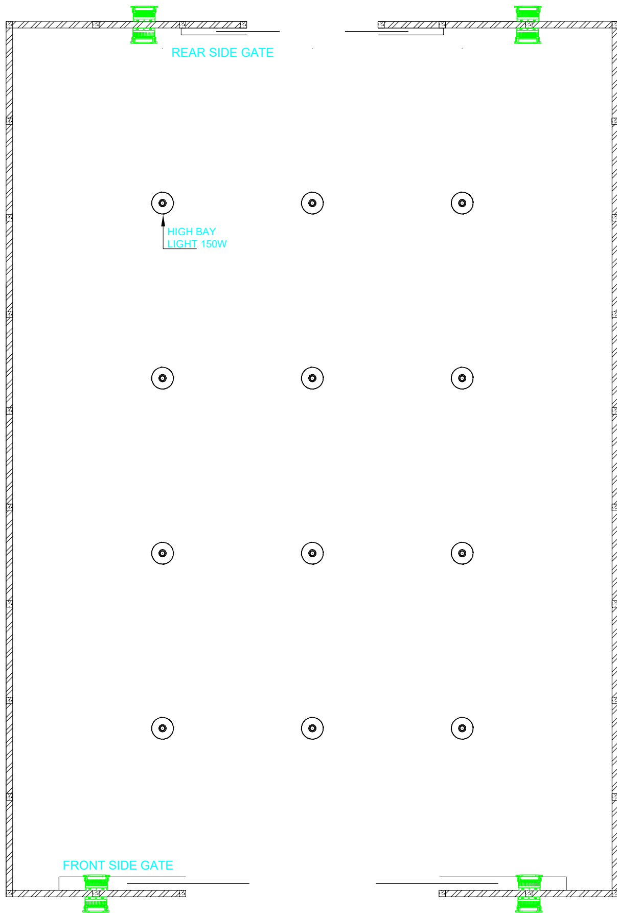
LIGHTING PLAN
