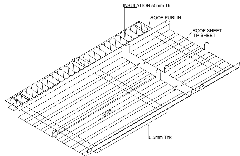
TP SHEET & ROOF PURLIN 3D VIEW DETAIL
