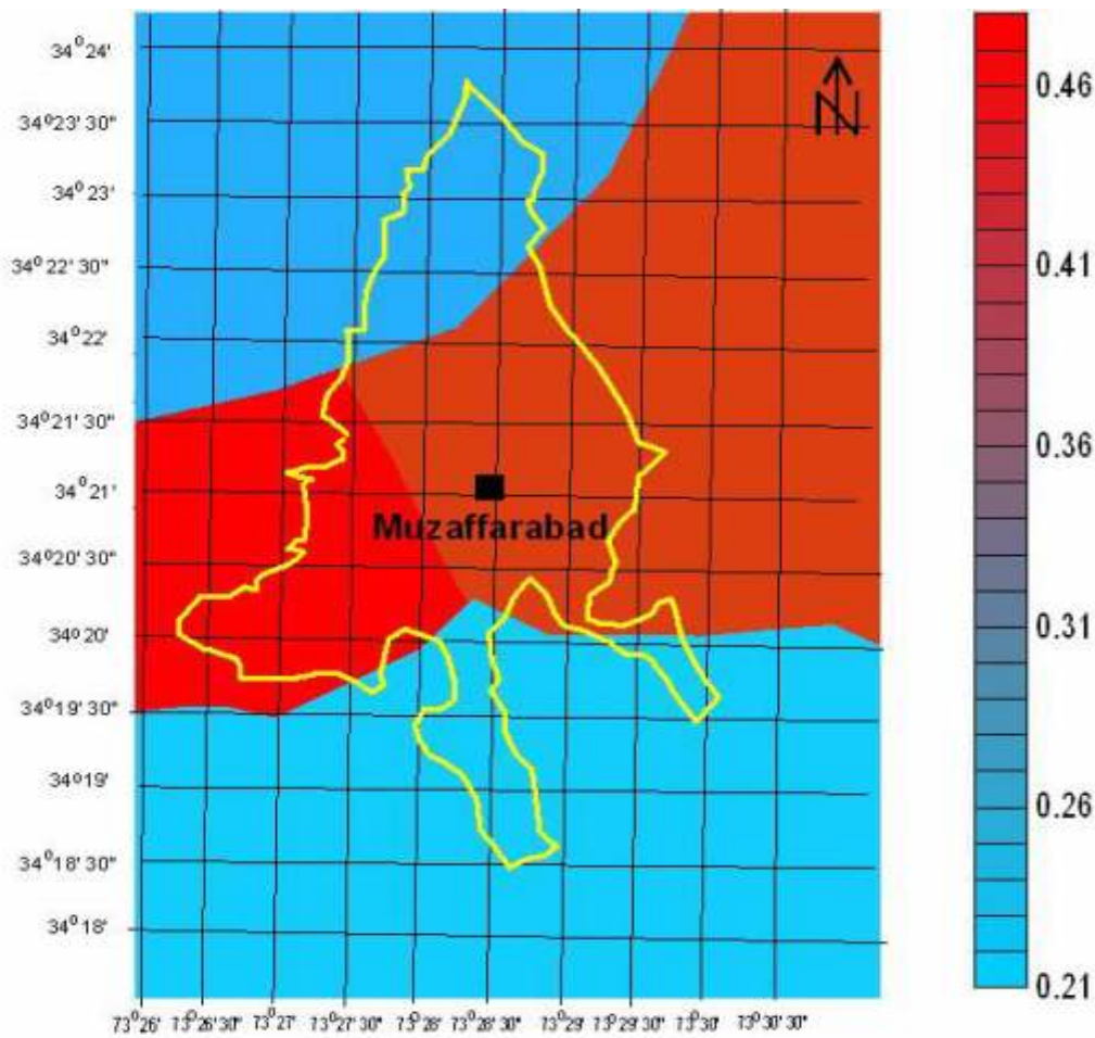
Fig. 11. Intensity based upon MMI scale, for Muzaffarabad.
