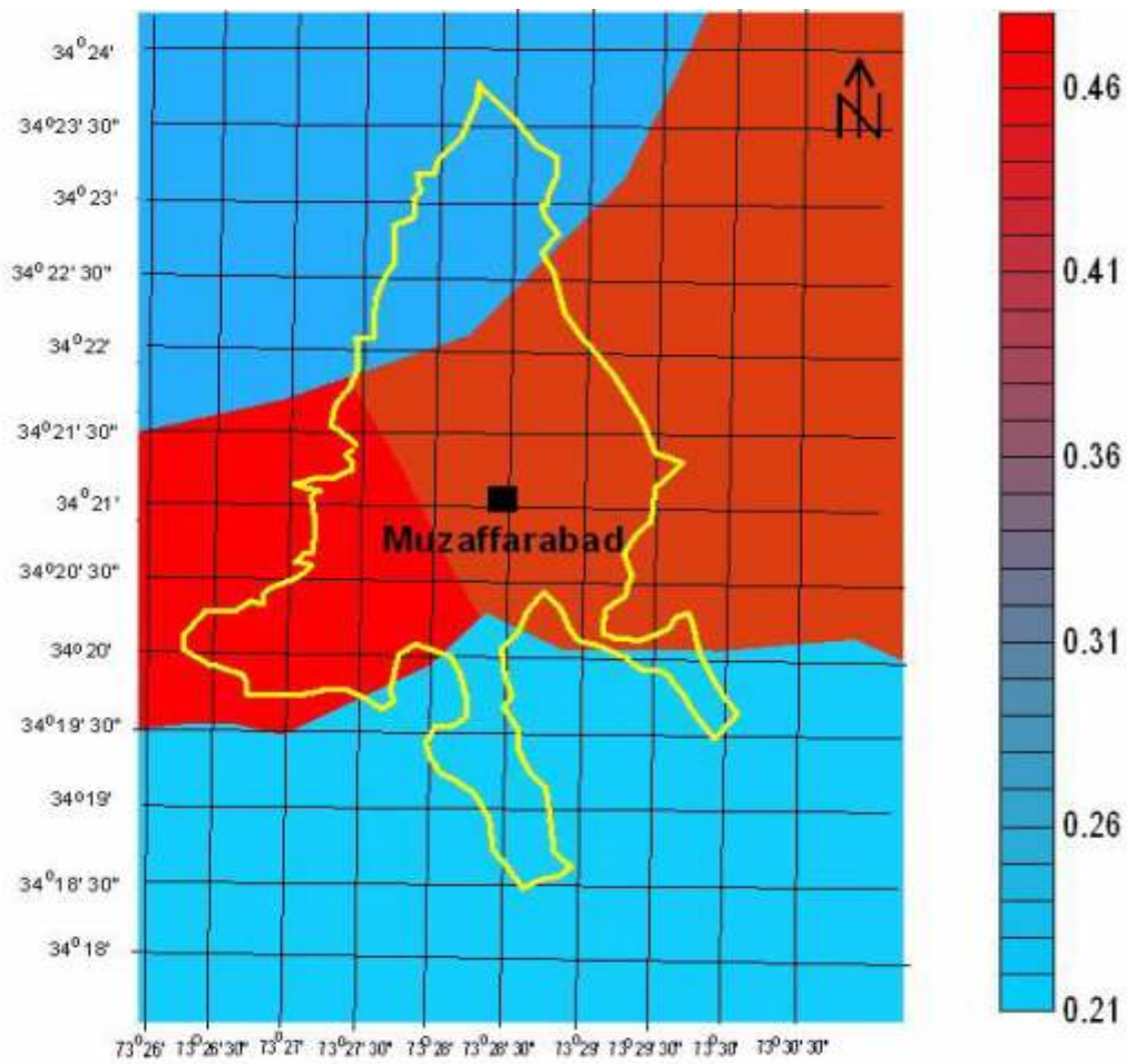
Fig. 10. Peak Ground Acceleration map for Muzaffarabad.
