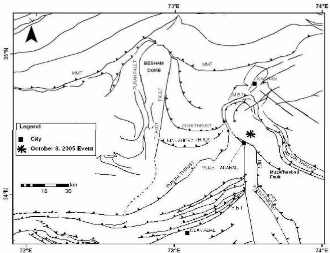
Fig.3. Structural map prepared in the present study (MonaLisa et al., 2008).
