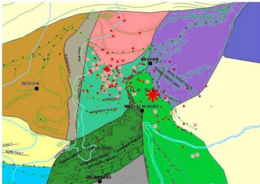
Fig7a. Seismotectonic map of the study area prepared in the present work (Closer view).
