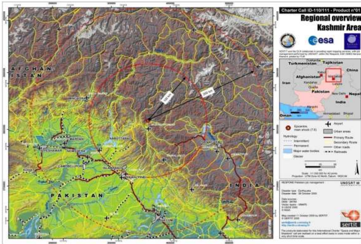
Fig.5. Regional overview of Kashmir area with Muzaffarabad Earthquake (UNOSAT, 2005).
