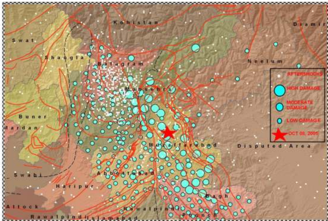
Fig.4. Major faults plotted on a satellite map, along with level of damage.
