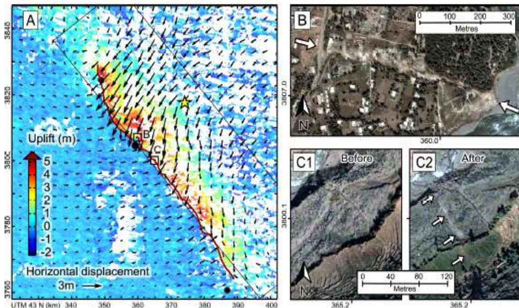
Fig.6. Field studies of the area surrounding Muzafarabad.
