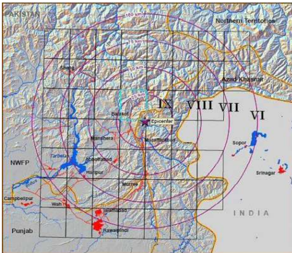
Fig. 9. Intensity map of Muzaffarabad and surrounding.
