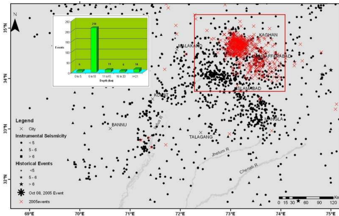
Fig.6. Seismicity map of the study area (MonaLisa et al., 2008).
