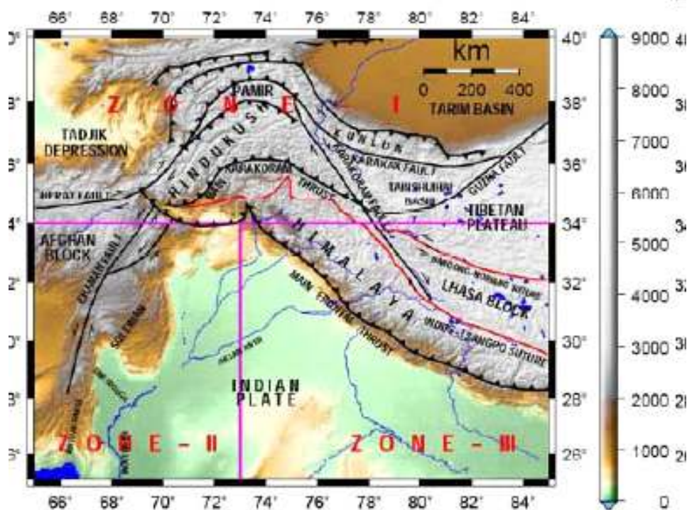
Figure 1. Tectonic setting of the study area.
