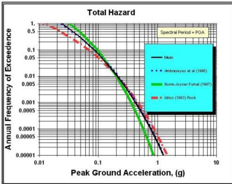
Fig. 8. Total seismic hazard curve for the site of Muzaffarabad for various return periods.
