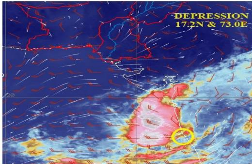
Satellite image (24 May 2025, 1000 PST)
