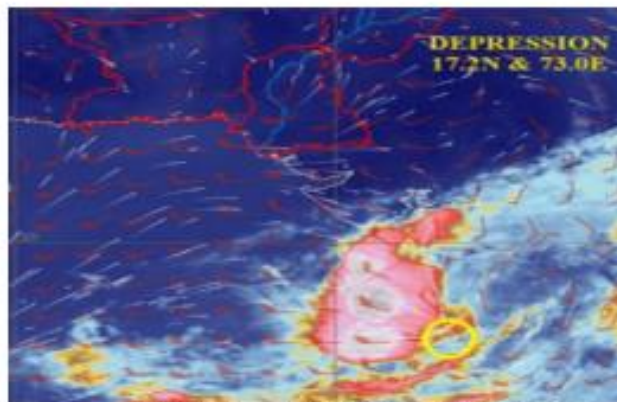
Satellite image (24 May 2025, 1000 PST)
