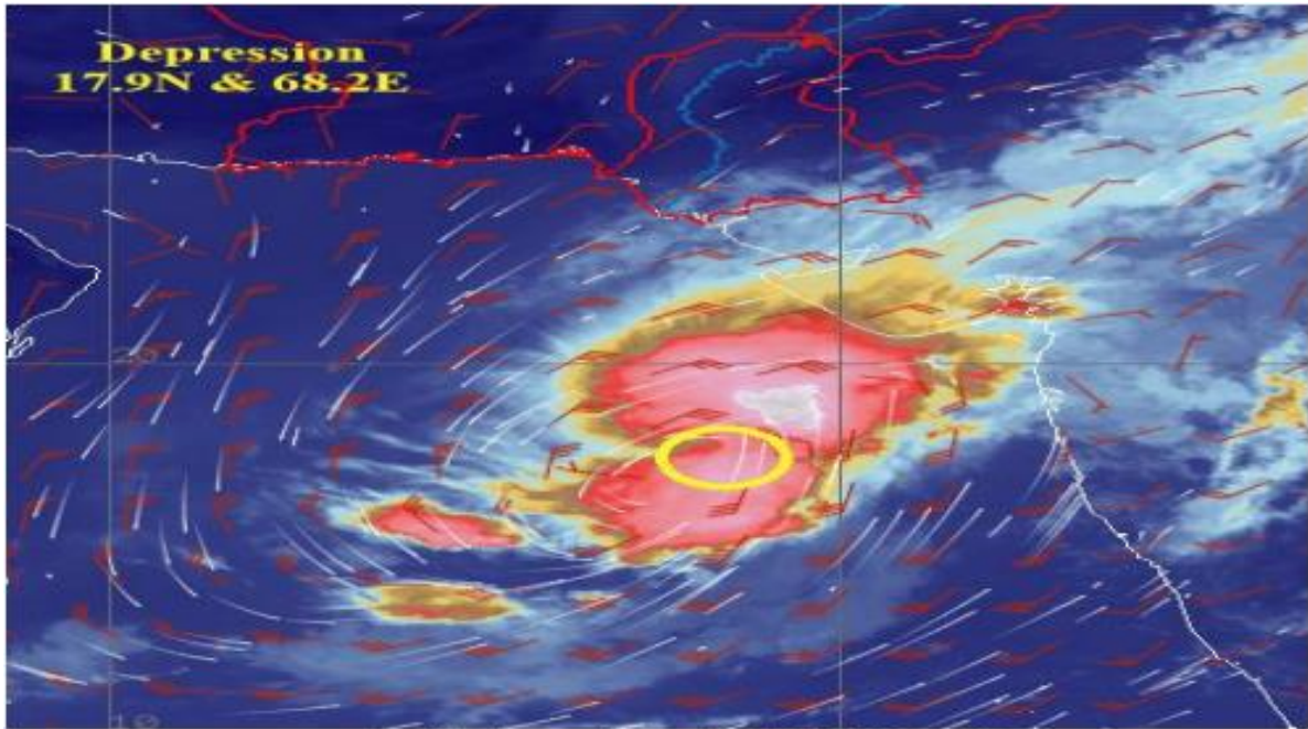
Satellite image (30 October 2025, 1030 PST)
