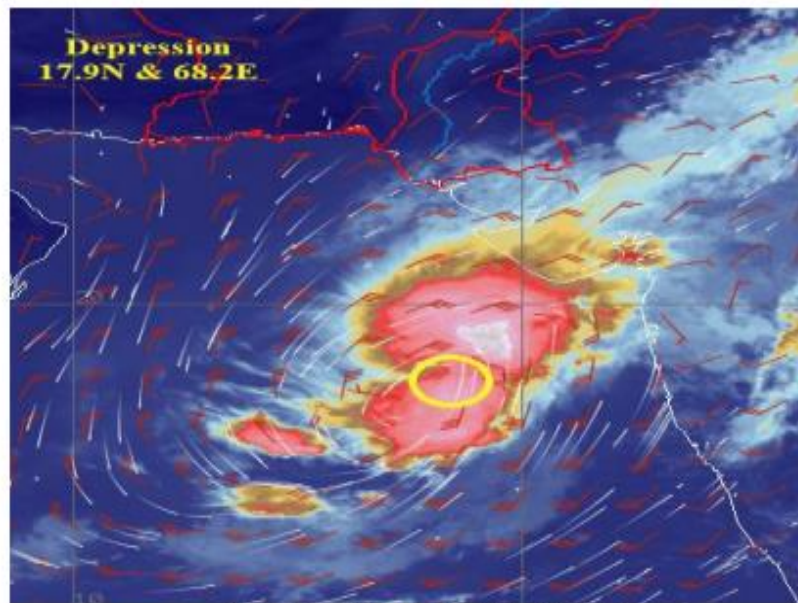
Satellite image (30 October 2025, 1030 PST)
