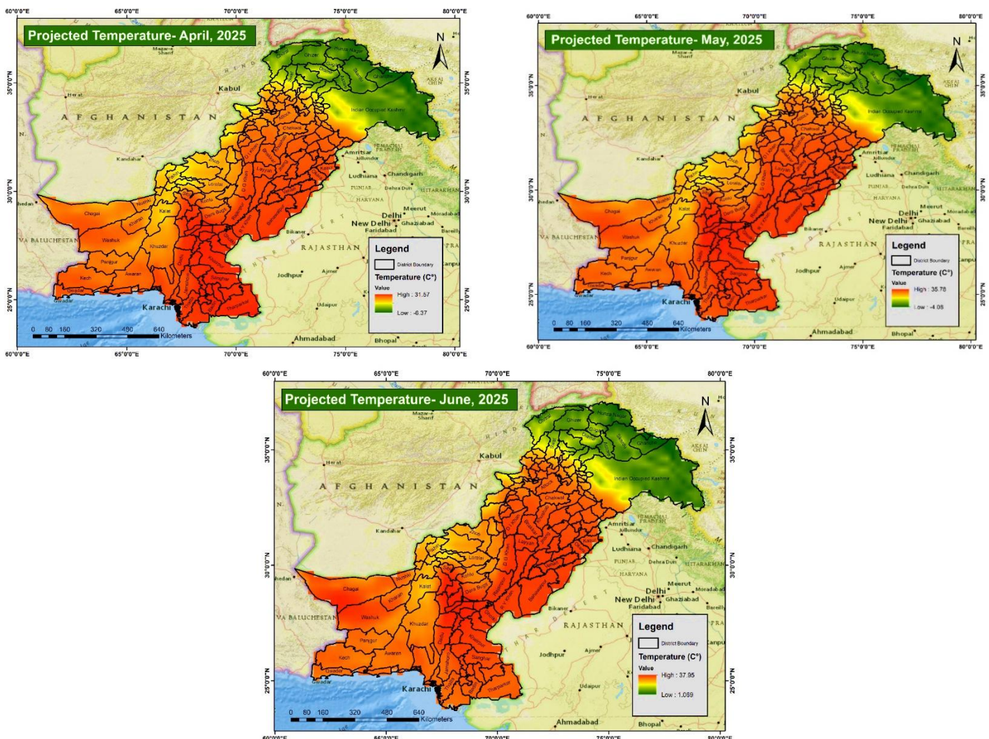
Figure: 6 Temperature Projection for the months of April, May and June 2025
